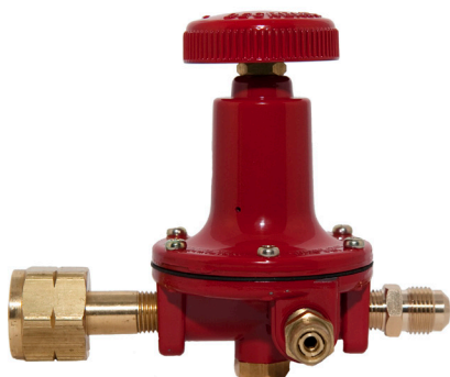
PART No. 1230LK2 0-30 PSI ADJUSTABLE Includes: liquid inlet fitting, relief valve, & 3/8" MSAE outlet fitting installed.
