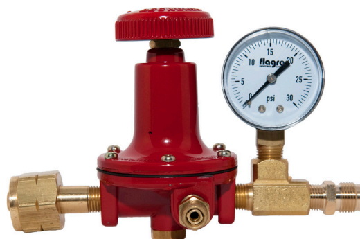
PART No. 1230LK4 0-30 PSI ADJUSTABLE Includes: liquid inlet fitting, tee, relief valve, pressure gauge & 3/8" MSAE outlet fitting installed.
