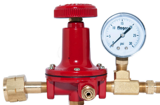
PART No. 1230LK3 0-30 PSI ADJUSTABLE Includes: liquid inlet fitting, tee, relief valve, pressure gauge & 9/16"-18 LH outlet fitting installed.
