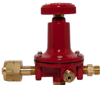
PART No. 1230LK1 0-30 PSI ADJUSTABLE Includes: liquid inlet fitting, relief valve, & 9/16"-18LH outlet fitting installed.
